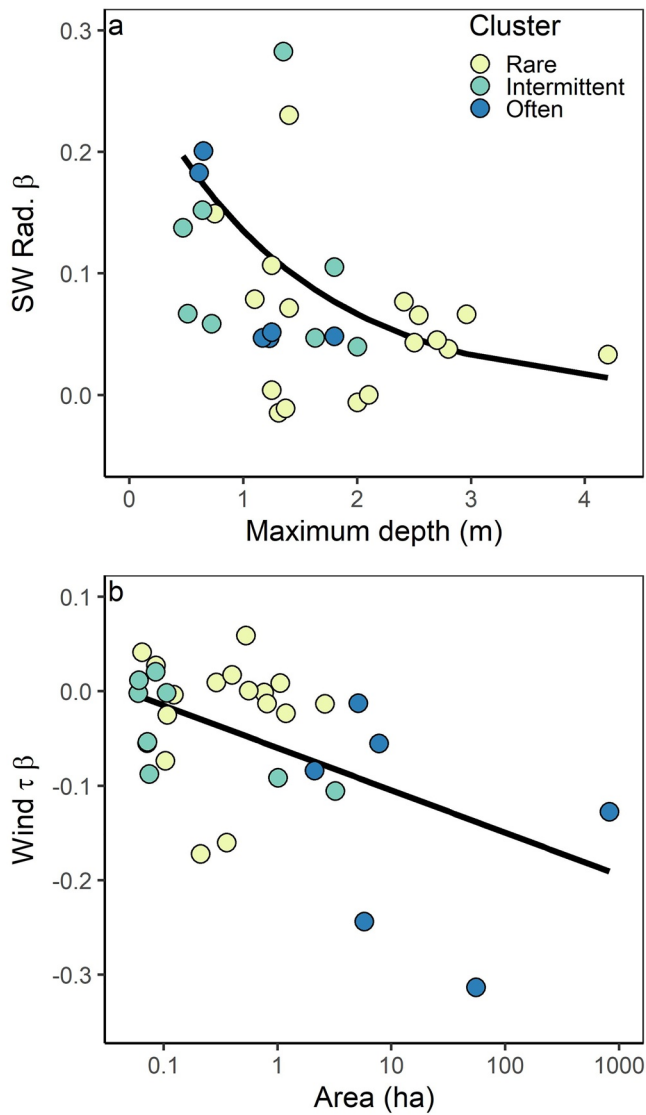
Figure 6. (a) Exponential relationship between the short wave radiation (SW Rad.) time series coefficient ( \beta between z -transformed total daily SW Rad. and daily mean density gradient) and maximum depth in each waterbody. (b) Linear relationship between wind shear stress (Wind \tau ) time series coefficient ( \beta between z -transformed max daily wind \tau and daily mean density gradient) and surface area in each waterbody. Sites are colored by mixing cluster (rare, intermittent, and often mixed). Black line indicates least-squares best fit regression line across all clusters.
